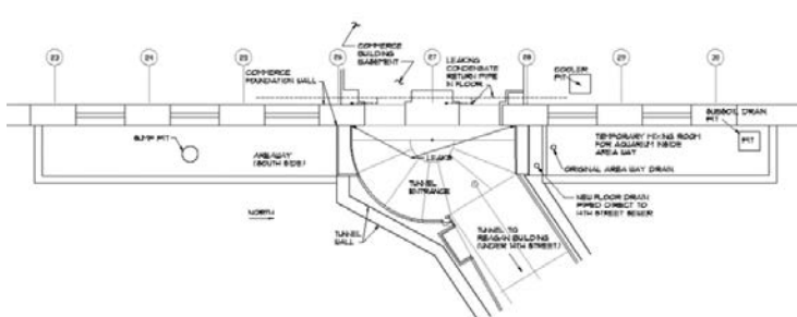
PLAN VIEW OF TUNNEL ENTRANCE INTO COMMERCE BUILDING
