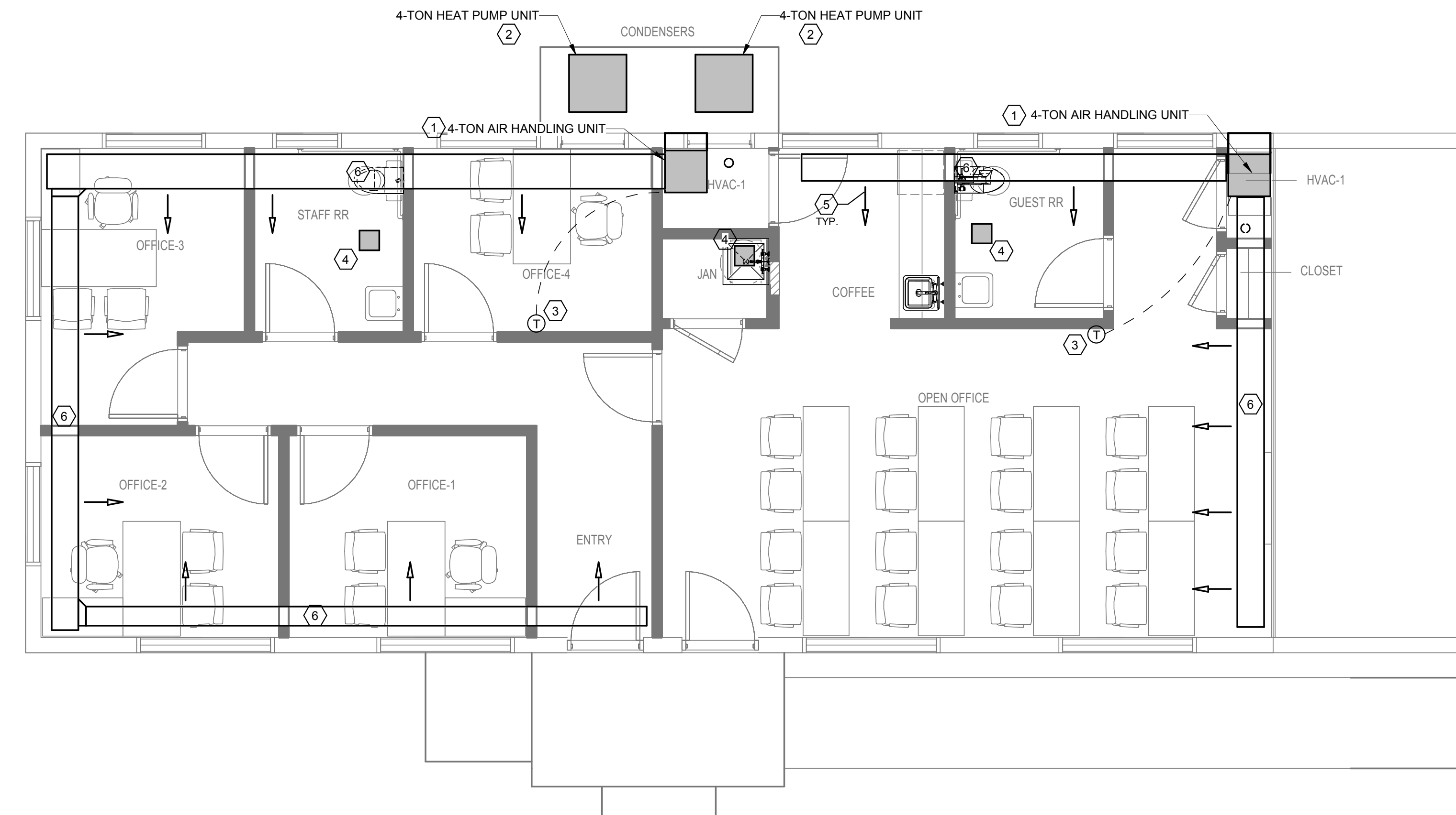
1 MECHANICAL FLOOR PLAN 1/4" = 1'-0"
