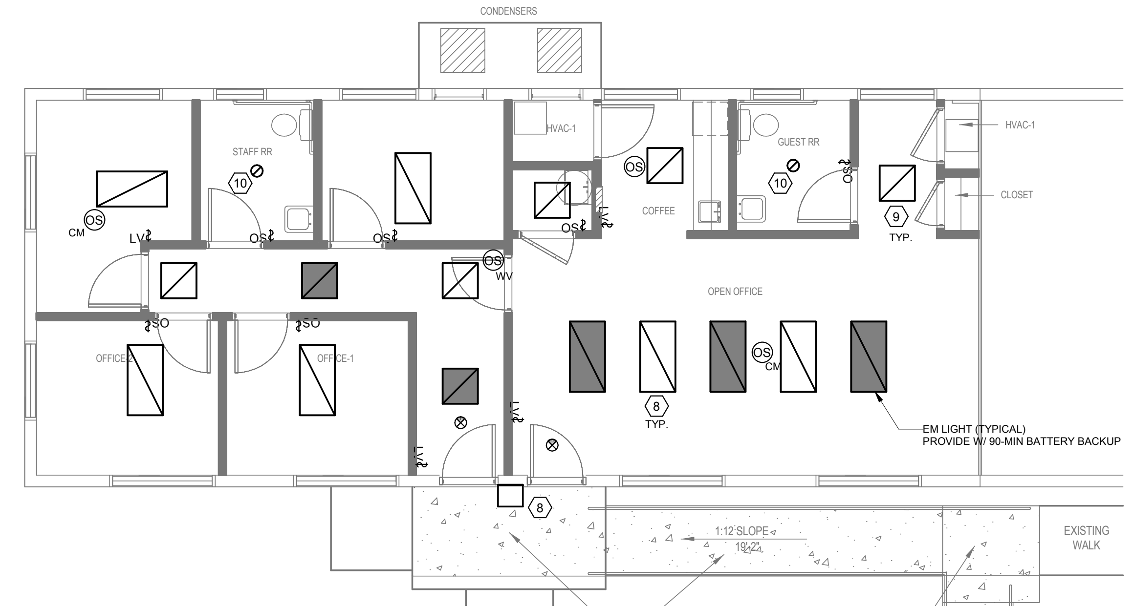
2 ELECTRICAL LIGHTING PLAN 3/16" = 1'-0"
