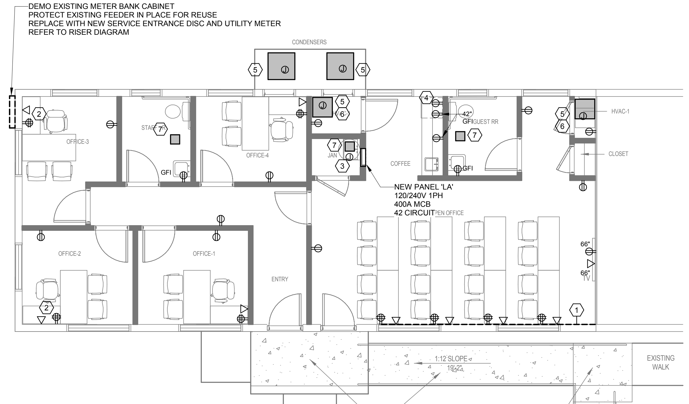
1 ELECTRICAL POWER PLAN 3/16" = 1'-0"
