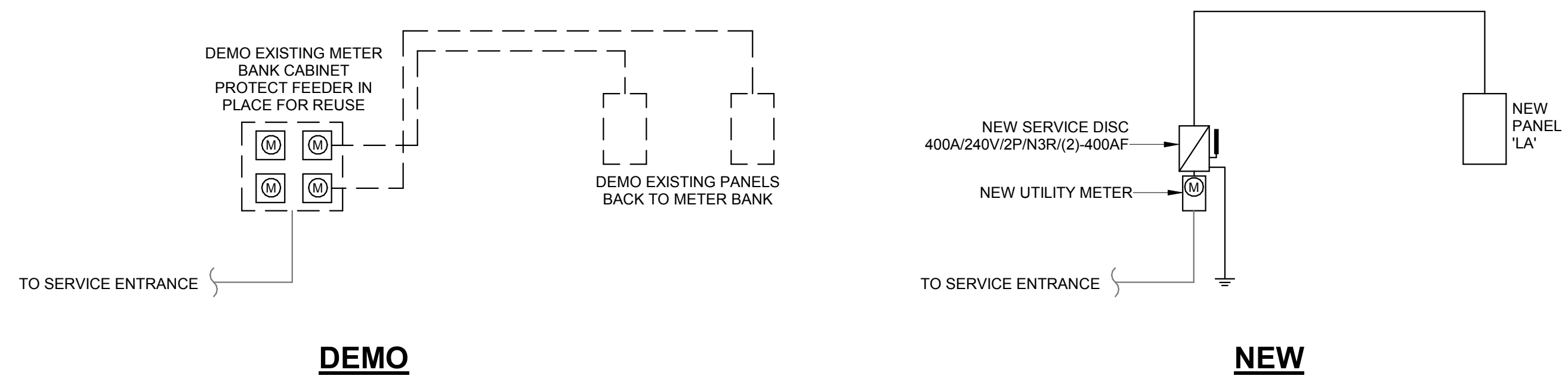
3 ELECTRICAL RISER DIAGRAM NOT TO SCALE
